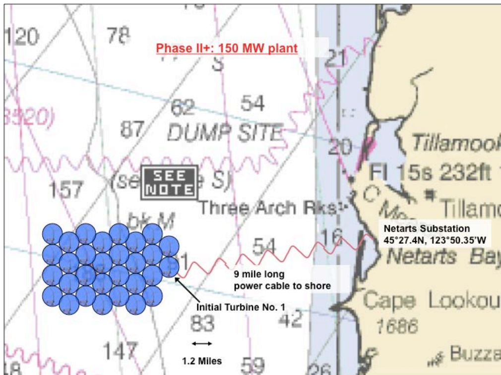
Figure 1-4 - Phase II+ plant footprint
