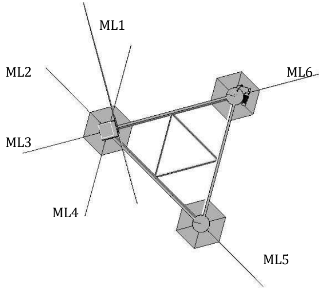
Figure 1-7: top view of the MF-Wind offshore wind turbine platform
