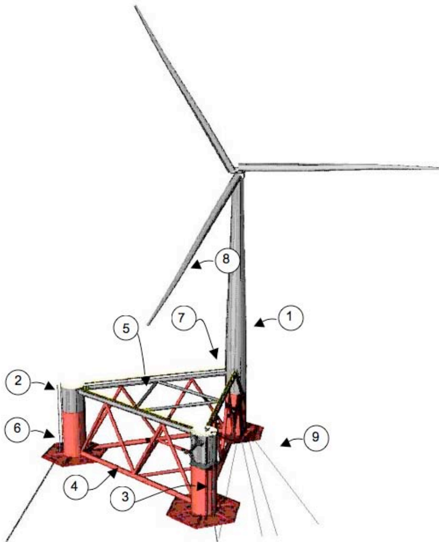
Figure 1-6 - WindFloat integrated with 5MW turbine
